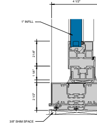
⑧ WINDOW SILL AT SILL WITH SEALANT OPTION & SILL FILLER CUP Ø = 1'-0"
