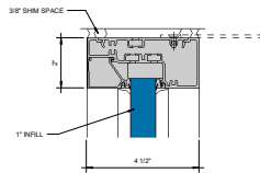
① HEAD W/STRAP ANCHOR 6" = 1'-0"
