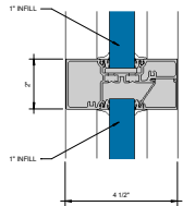
5 HORIZONTAL 6" = 1'-0"
