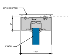
① HEAD W/ STRAP ANCHOR G = 1'-0"
