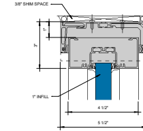
HW COMPENSATING RECEPTOR FOR OUTSIDE GLAZED HEAD GLASS STOPS ④ \frac{1}{2}''
