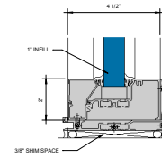
③ SILL WITH SEALANT OPTION Ø = 1'-0"
