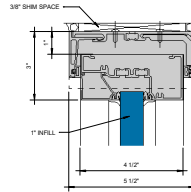
HW COMPENSATING RECEPTOR FOR OUTSIDE GLAZED HEAD ② \frac{1}{2}''
