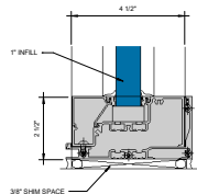
⑨ SILL WITH SEALANT & GASKET OPTION 6" = 1'-0"
