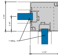
90° INSIDE CORNER TWO POCKETS Ø = 1-0"
