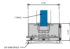
⑥ SILL WITH SILL FILLER CLIP, SEALANT & GASKET OPTION S' = 1'-0"
