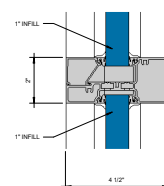
③ HORIZONTAL G = 1'-0"
