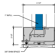
⑦ SILL WITH SEALANT OPTION 6" = 1'-0"
