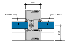
⑦ VERTICAL MULLION 6" = 1'-0"
