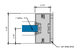
⑧ LAST BAY JAMB G = 1'-0"
