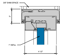
② HEAD W/RECEPTOR 6" = 1'-0"
