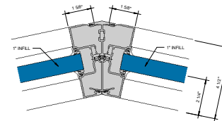
ADJUSTABLE PIVOT INSIDE CORNER Ø = 1-0"
