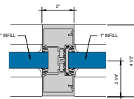
⑩ HEAVY WEIGHT MULLION Ø = 1'-0"
