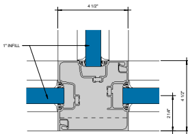
CORNER POST AT JAMB WITH ONE POCKET DETAIL Ø = 1-0"
