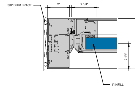
⑪ CASEMENT OUTSWING 6" = 1'-0"
