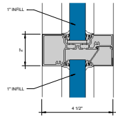
⑤ HORIZONTAL 6" = 1'-0"
