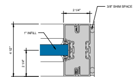
⑧ LAST BAY JAMB S 1 = 1'-0"
