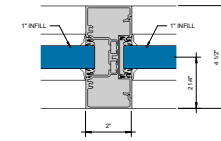
⑧ VERTICAL MULLION S' = 1'-0"
