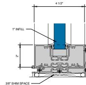
⑥ SILL WITH SILL FILLER CLIP, SEALANT & GASKET OPTION-3C-3 Ø = 1'-0"
