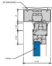
① WINDOW HEAD AT HEAD Ø = 1'-0"
