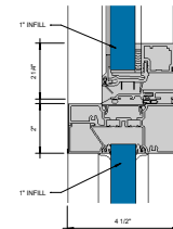
③ CASEMENT OUTSWING 6" = 1'-0"
