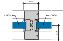
⑪ 2 1/4" VERTICAL MULLION 6" = 1'-0"
