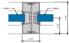
① EXPANSION MULLION S 1 = 1'-0"
