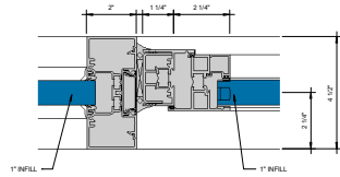
① VERTICAL MULLION S=1-10
