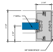
③ LAST BAY JAMB W/ STEEL 6" x 1'-0"
