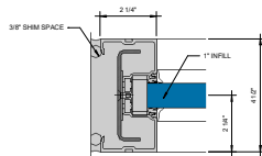
FIRST BAY JAMB WITH STEEL REINFORCEMENT ① 6" x 1'-0"
