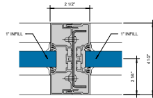
② EXPANSION MULLION WITH STEEL E = 1-0"
