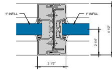
② EXPANSION MULLION WITH STEEL S 1 = 1'-0"
