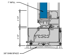
PROJECT OUT - SILL WITH SEALANT ⑥ OPTION 6" = 1'-0"
