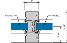
⑧ VERTICAL MULLION 6" = 1'-0"
