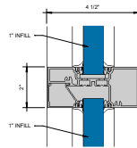
② HORIZONTAL S' = 1'-0"
