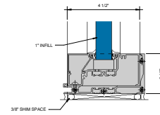
③ SILL WITH SEALANT OPTION S' = 1'-0"
