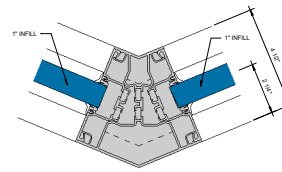
135° OUTSIDE CORNER Ø = 1-0"
