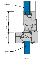
③ WINDOW SILL AT HORIZONTAL Ø = 1'-0"
