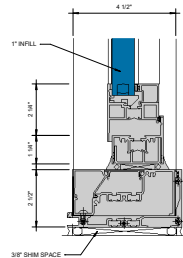
⑥ WINDOW SILL AT SILL WITH SEALANT OPTION Ø = 1'-0"
