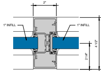
⑨ MEDIUM WEIGHT MULLION 6" = 1'-0"
