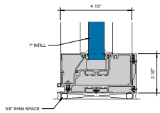
⑤ SILL WITH SEALANT & GASKET OPTION S' = 1'-0"
