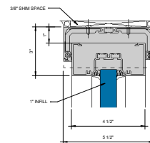
HW ONE PIECE COMPENSATING HEAD RECEPTOR FOR OUTSIDE GLAZED HEAD GLASS STOPS "UP" ⑨ \frac{1}{2}''
