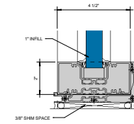
④ SILL WITH SILL FILLER CLIP, SEALANT & GASKET OPTION-3A-3 Ø = 1'-0"
