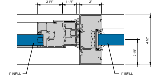
12 VERTICAL MULLION 6" = 1'-0"
