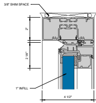
① HEAD CASEMENT OUTSWING 6" = 1'-0"
