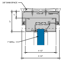
COMPENSATING RECEPTOR FOR INSIDE GLAZED HEAD ⑤ \frac{1}{2}''
