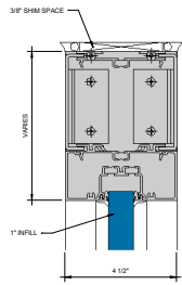
Ⓒ BRAKE METAL ADAPTER OUTSIDE GLAZED HEAD 6" = 1'-0"
