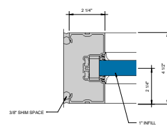
⑥ FIRST BAY JAMB S 1 = 1'-0"
