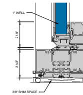
PROJECT OUT - SILL WITH SEALANT ⑧ OPTION & SILL FILLER CLIP 6" = 1'-0"
