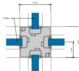
CORNER POST FOUR POCKETS Ø = 1-0"
