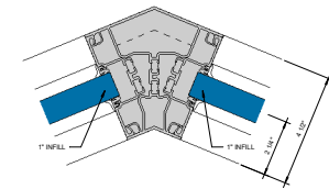
135° INSIDE CORNER Ø = 1-0"
