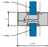
② HORIZONTAL 6" = 1'-0"
