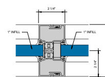
⑦ VERTICAL MULLION S 1 = 1'-0"
