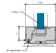
④ SILL WITH SCREW DOWN S 1 = 1'-0"
