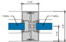
① EXPANSION MULLION R 1 = 1.0"
