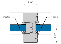
⑪ 2-1/4" VERTICAL MULLION Ø = 1'-0"
