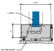
⑤ SILL WITH SEALANT & GASKET OPTION 6" = 1'-0"
