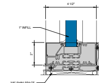
④ SILL WITH SILL FILLER CLIP, SEALANT & GASKET OPTION 6" = 1'-0"
