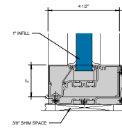
④ SILL WITH SCREW DOWN 6" = 1'-0"
