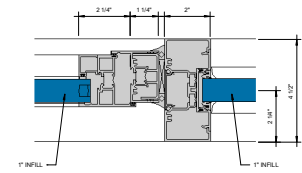
⑫ VERTICAL MULLION Ø = 1'-0"
