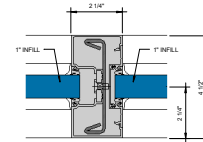
⑫ 2-1/4" VERTICAL MULLION WITH STEEL Ø = 1'-0"
