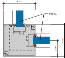
90° OUTSIDE CORNER TWO POCKETS Ø = 1-0"
