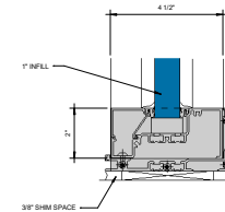
④ SILL WITH SCREW DOWN G = 1'-0"
