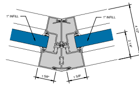
ADJUSTABLE PIVOT OUTSIDE CORNER Ø = 1-0"
