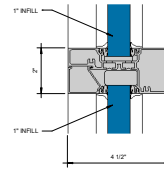
③ HORIZONTAL 6" = 1'-0"
