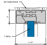
② HEAD 6" = 1'-0"
