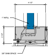
⑨ SILL WITH SEALANT & GASKET OPTION Ø = 1'-0"
