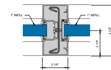
⑫ 2-1/4" VERTICAL MULLION WITH STEEL S' = 1'-0"
