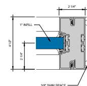
⑧ LAST BAY JAMB 6" = 1'-0"
