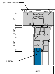
① WINDOW HEAD AT HEAD Ø = 1'-0"
