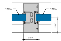
⑪ 2-1/4" VERTICAL MULLION S' = 1'-0"
