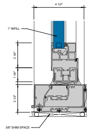
⑥ WINDOW SILL AT SILL WITH SEALANT OPTION Ø = 1'-0"
