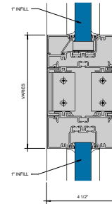
Ⓒ BRAKE METAL ADAPTER OUTSIDE GLAZED HORIZONTAL 6" = 1'-0"
