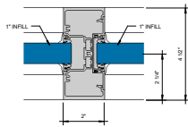
⑨ MEDIUM WEIGHT MULLION S' = 1'-0"
