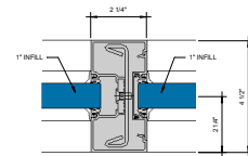
⑫ 2 1/4" VERTICAL MULLION WITH STEEL 6" = 1'-0"
