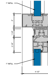
④ WINDOW HEAD AT HORIZONTAL Ø = 1'-0"
