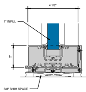
⑤ SILL WITH SILL FILLER CLIP G = 1'-0"
