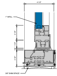
⑧ WINDOW SILL AT SILL WITH SEALANT OPTION & SILL FILLER CLIP Ø = 1'-0"
