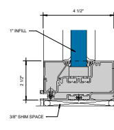
7 SILL WITH SEALANT OPTION 6" = 1'-0"
