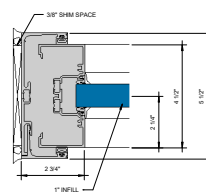
COMPENSATING RECEPTOR FOR OUTSIDE GLAZED JAMB ⑪ \frac{1}{2}''
