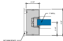
⑥ FIRST BAY JAMB 6" = 1'-0"
