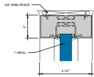
① HEAD 6" = 1'-0"
