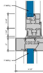
3 WINDOW SILL AT HORIZONTAL 6" = 1'-0"
