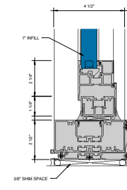
8 WINDOW SILL AT SILL WITH SEALANT OPTION & SILL FILLER CLIP 6" = 1'-0"
