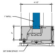
⑤ SILL WITH SEALANT & GASKET OPTION-3B-3 Ø = 1'-0"
