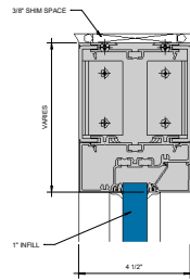
Ⓒ BRAKE METAL ADAPTER INSIDE GLAZED HEAD 6" = 1'-0"
