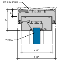
COMPENSATING RECEPTOR FOR OUTSIDE GLAZED HEAD ① \frac{1}{2}''
