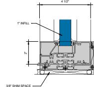
⑥ SILL WITH SILL FILLER CLIP, SEALANT & GASKET OPTION 6" = 1'-0"
