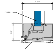
⑦ SILL WITH SEALANT OPTION Ø = 1'-0"
