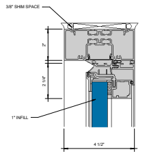
① HEAD CASEMENT OUTSWING 6" = 1'-0"
