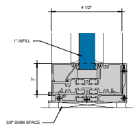
⑤ SILL WITH SILL FILLER CLIP S 1 = 1'-0"
