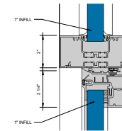
④ PROJECT OUT 6" = 1'-0"
