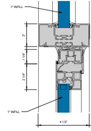
④ WINDOW HEAD AT HORIZONTAL Ø = 1'-0"
