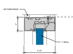
① HEAD W/STRAP ANCHOR S 1 = 1'-0"
