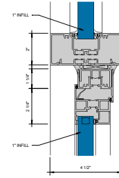
4 WINDOW HEAD AT HORIZONTAL 6" = 1'-0"
