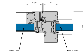
⑫ CASEMENT OUTSWING 6" = 1'-0"
