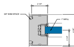
⑥ FIRST BAY JAMB G = 1'-0"
