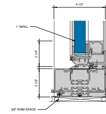
⑧ PROJECT-OUT-SILL WITH SEALANT OPTION & SILL FILLER CLIP 6" = 1'-0"
