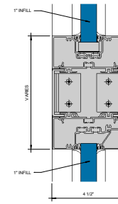
Ⓒ BRAKE METAL ADAPTER INSIDE GLAZED HORIZONTAL 6" = 1'-0"
