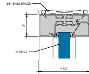
② HEAD 6" = 1'-0"
