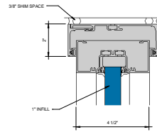
② HEAD W/ RECEPTOR G = 1'-0"
