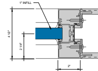
Ⓒ TOP VIEW BRAKE METAL ADAPTER 6" = 1'-0"
