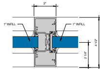
⑨ MEDIUM WEIGHT MULLION Ø = 1'-0"
