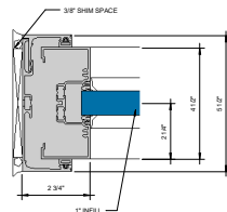
COMPENSATING RECEPTOR FOR OUTSIDE GLAZED JAMB ⑩ \frac{1}{2}''
