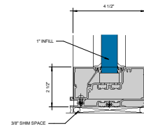
⑦ SILL WITH SEALANT OPTION 6" = 1'-0"
