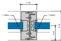
② EXPANSION MULLION WITH STEEL R 1 = 1.0"
