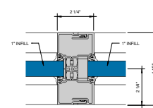
⑦ VERTICAL MULLION G = 1'-0"
