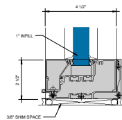
⑨ SILL WITH SEALANT & GASKET OPTION Ø = 1'-0"
