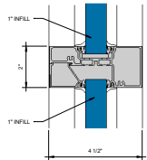
⑤ HORIZONTAL 6" = 1'-0"
