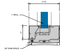
③ SILL WITH SEALANT OPTION 6" = 1'-0"
