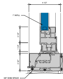
6 WINDOW SILL AT SILL WITH SEALANT OPTION 6" = 1'-0"
