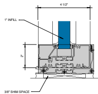
⑤ SILL WITH SILL FILLER CLIP 6" = 1'-0"
