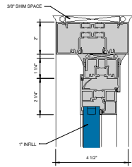
1 WINDOW HEAD AT HEAD 6" = 1'-0"
