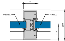
⑩ HEAVY WEIGHT MULLION 6" = 1'-0"
