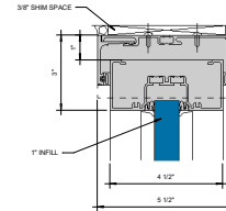
COMPENSATING RECEPTOR FOR OUTSIDE GLAZED HEAD GLASS STOPS ③ \frac{1}{2}''
