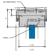
HW COMPENSATING RECEPTOR FOR INSIDE GLAZED HEAD ⑥ \frac{1}{2}''
