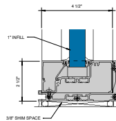
9 SILL WITH SEALANT & GASKET OPTION 6" = 1'-0"
