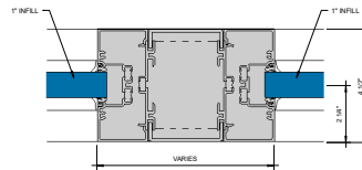
Ⓒ BRAKE METAL ADAPTER VERTICAL 6" = 1'-0"
