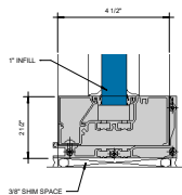
SILL WITH SEALANT AND GASKET ⑨ OPTION 6" = 1'-0"
