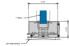
④ SILL WITH SILL FILLER CUP, SEALANT OPTION S' = 1'-0"
