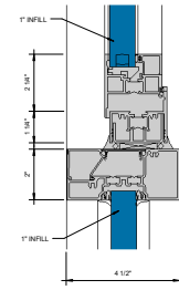
③ WINDOW SILL AT HORIZONTAL Ø = 1'-0"
