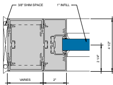
Ⓒ BRAKE METAL ADAPTER JAMB 6" = 1'-0"
