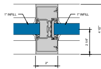
⑩ HEAVY WEIGHT MULLION S' = 1'-0"
