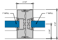
① EXPANSION MULLION E = 1-0"
